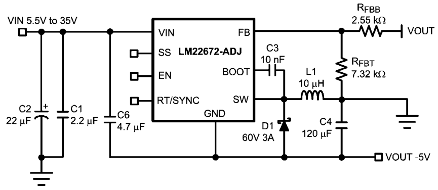
FIGURE 12. Inverting Regulator Application
