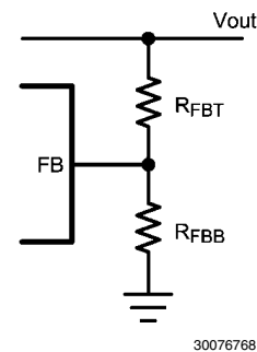
FIGURE 10. Output Voltage Divider
