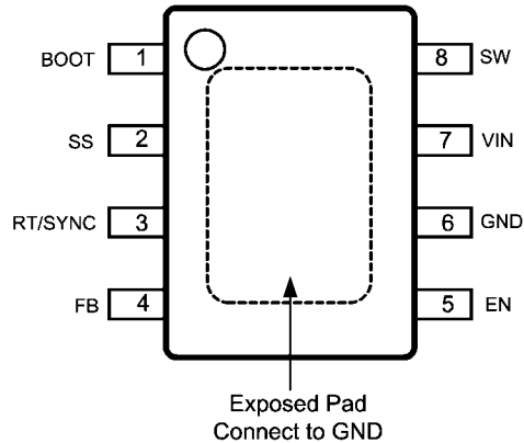
30076740 8-Lead Plastic PSOP-8 Package TI Package Number MRA08B
