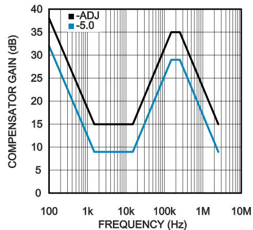
FIGURE 8. Compensator Gain
